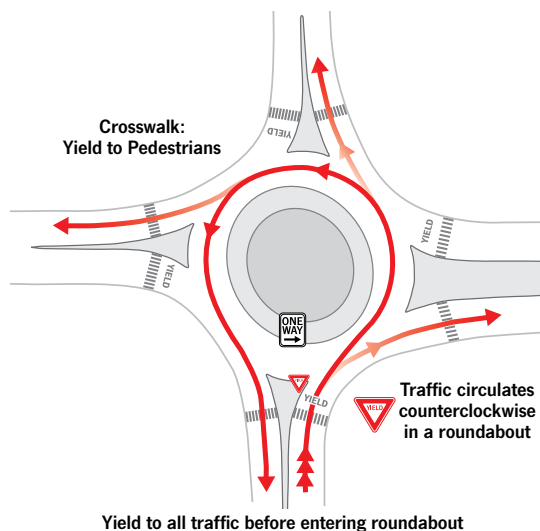
This example shows the traffic movement patterns through a one-lane roundabout. The one-lane roundabout is known as one of the safest and most efficient intersections.
